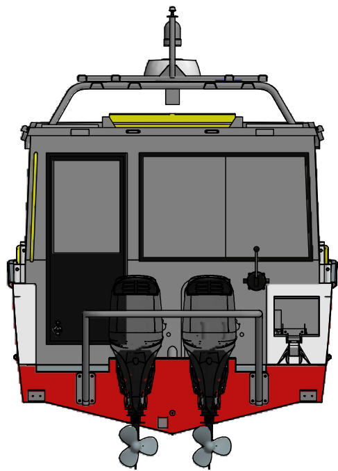
REAR VIEW ( 1 :50 )
