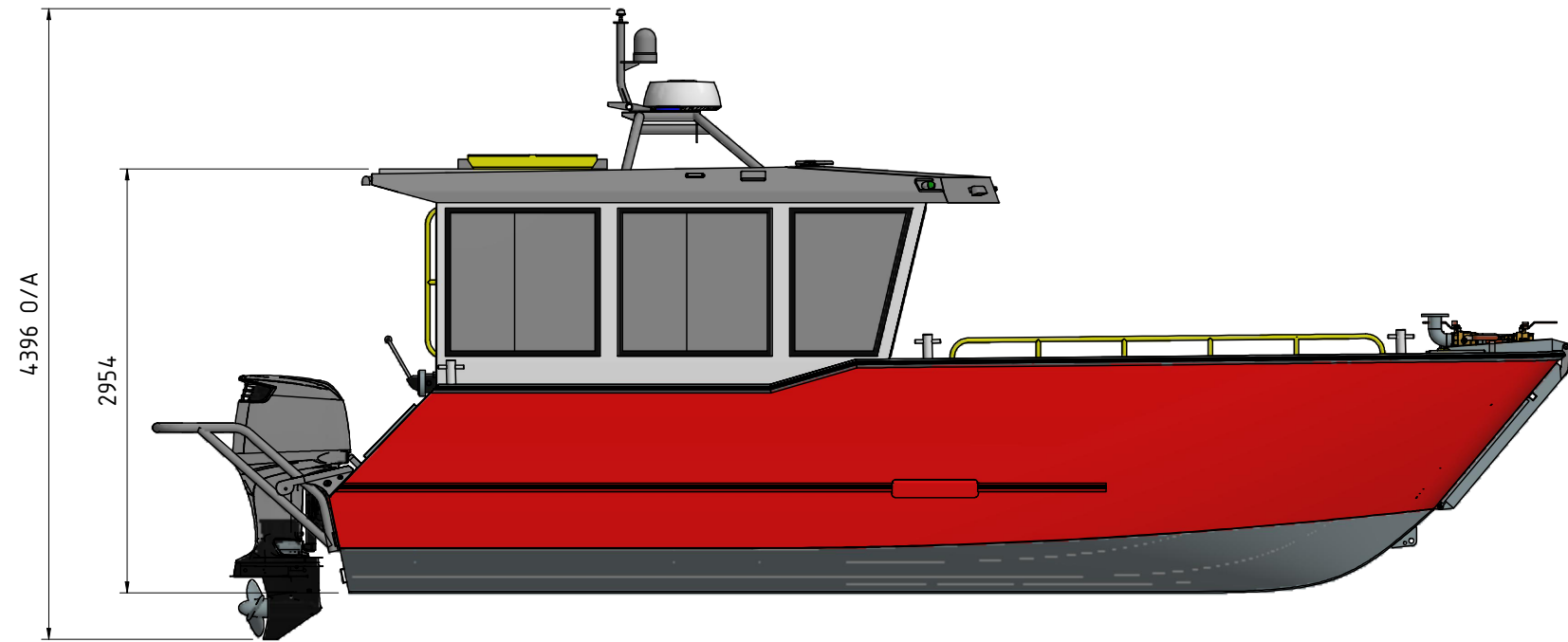
ELEVATION ( 1 :50 )
