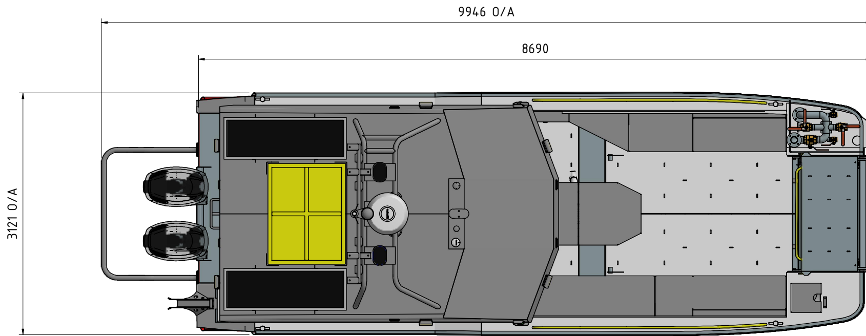
PLAN ( 1 :50 )
