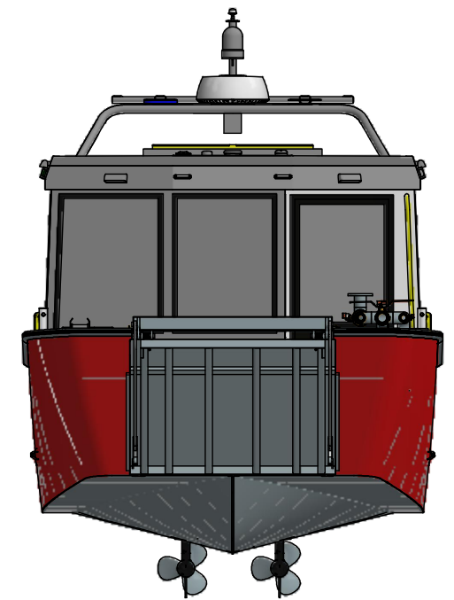
FRONT VIEW ( 1 :50 )
